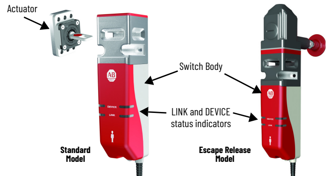
Figure 1 – Assembly Overview
