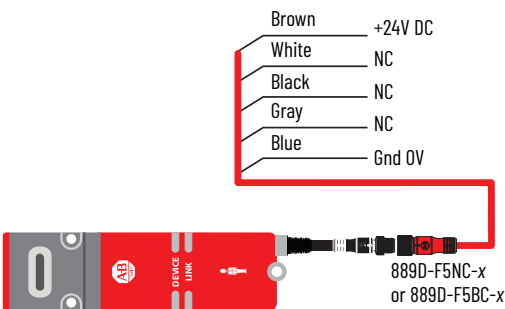
Figure 7 - Wiring
