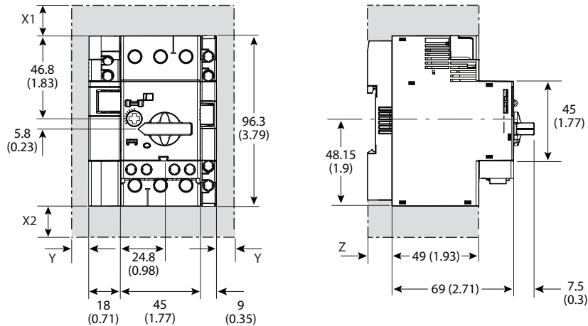
Figure 12 - Spacing Requirements
